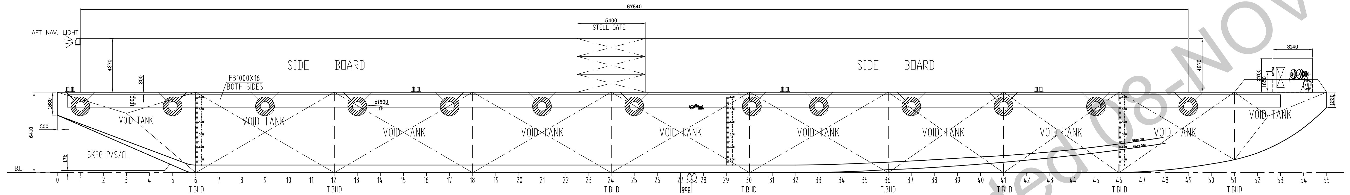
OUTBOARD PROFILE
